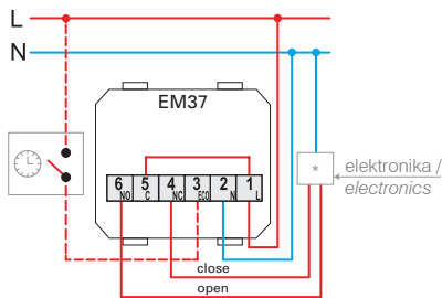
motorni pogon (omejena uporaba pri talnem ogrevanju) / motor drive (limited use with underfloor heating)
